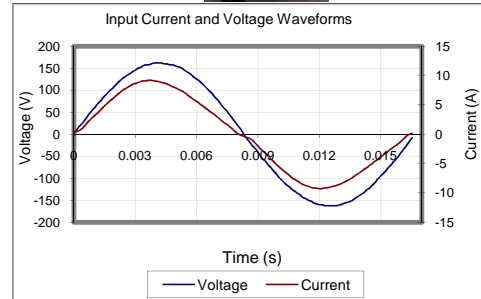
Input AC Current Waveform (ITHD = 10.54%, 50% Load)
