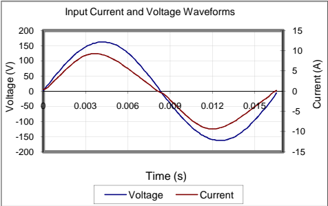
Input AC Current Waveform (ITHD = 9.98%, 50% Load)
